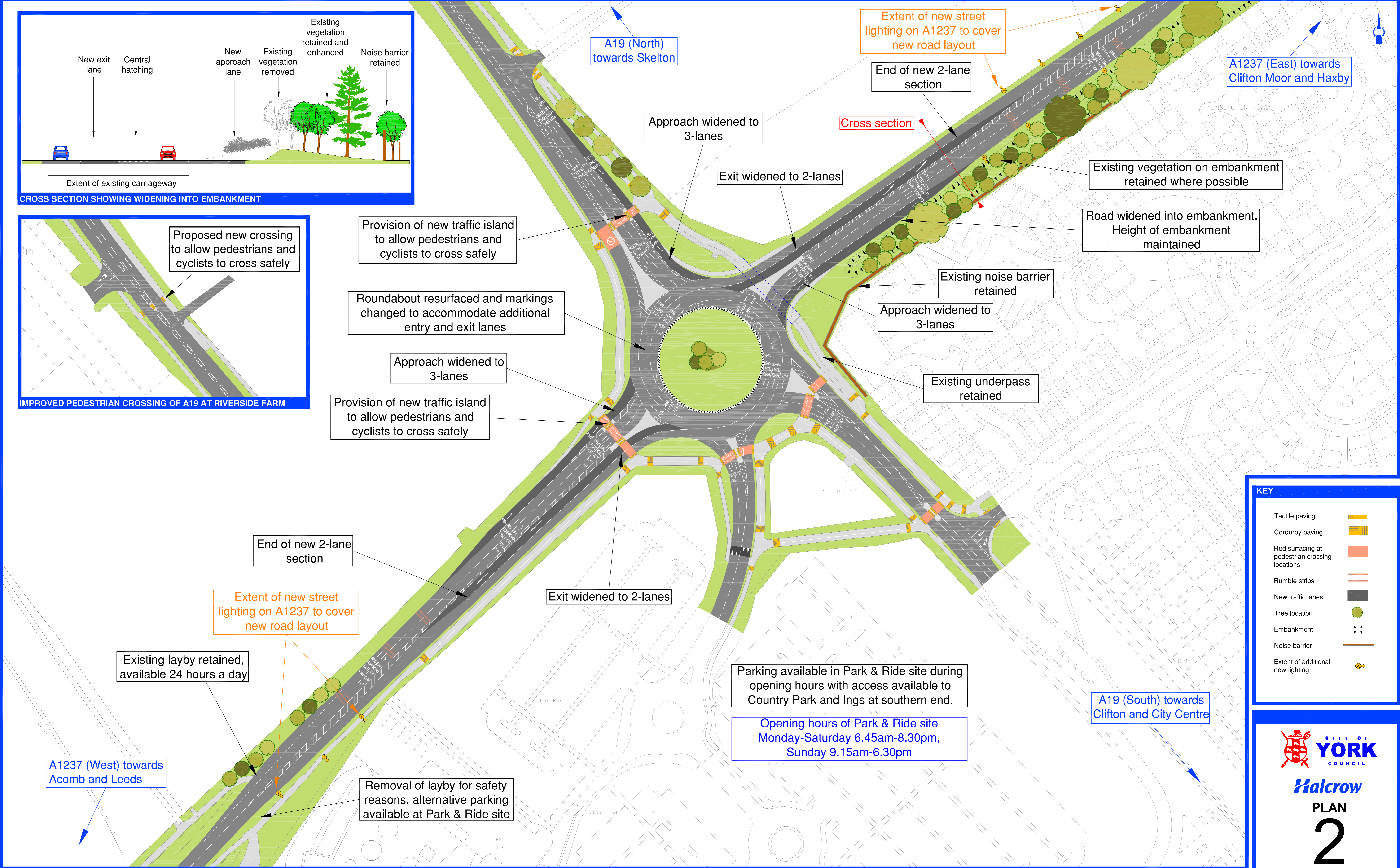
A19/A1237 RAWCLIFFE ROUNDABOUT PROPOSED LAYOUT
